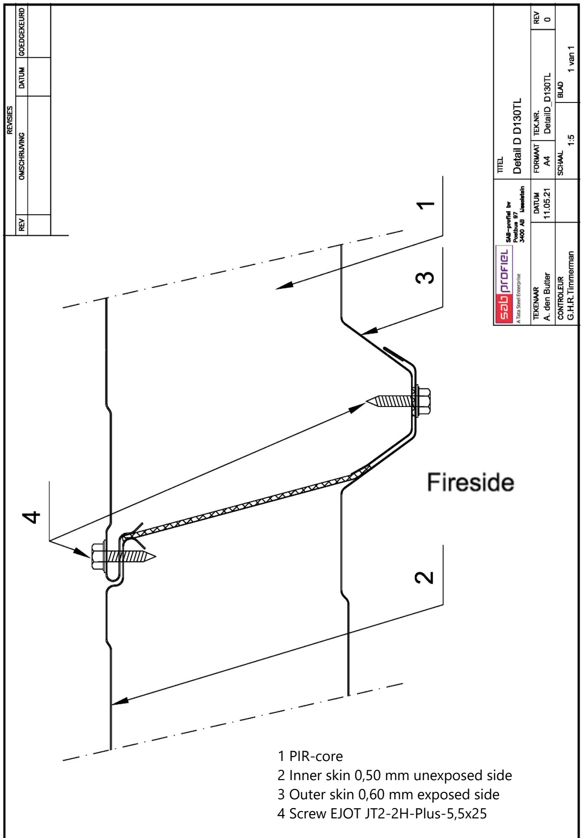
Figure 5: Detail connection between sandwich panels
